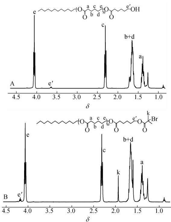
Fig. 2 (A) ^1\text{H-NMR} spectrum of \text{LPCL}_{20} in \text{CDCl}_3 and (B)
