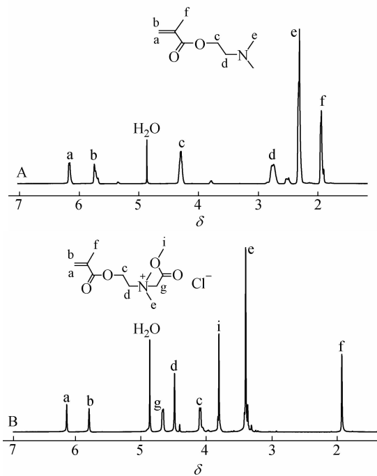
Fig. 3 (A) ^1\text{H-NMR} spectrum of DMA in \text{D}_2\text{O} and (B)
