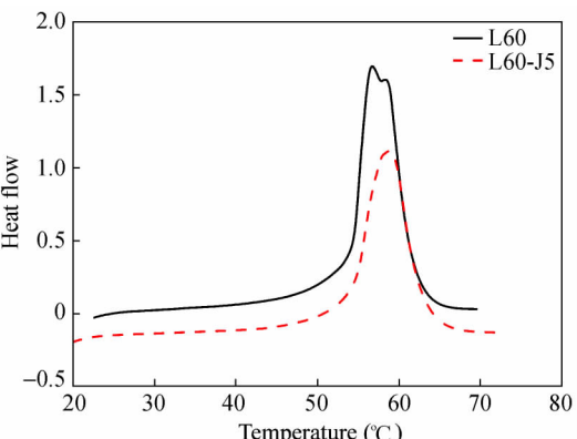
Fig. 5 DSC curves of LPCL and LPCL-PJDMA
