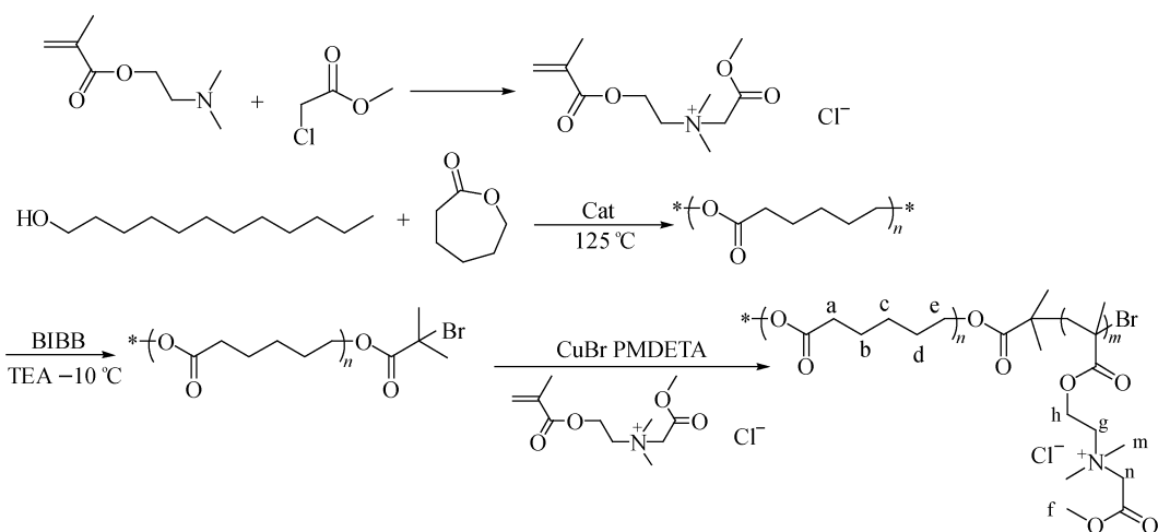
Fig. 1 Synthesis route to LPCL-PJDMA diblock copolymer
