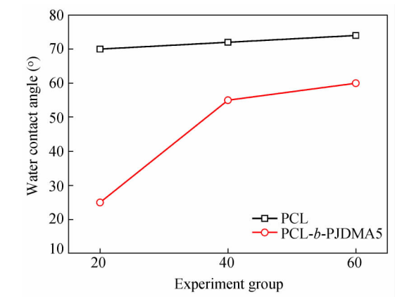
Fig. 6 Water contact angle of LPCL and LPCL-PJDMA
